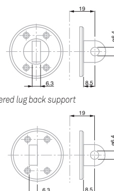
Off-centered lug back support
