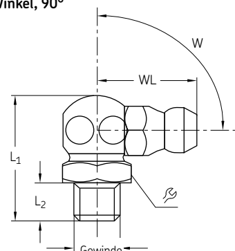
Winkel, 90°
