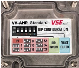
Fig. 4: Preamplifier electronics
