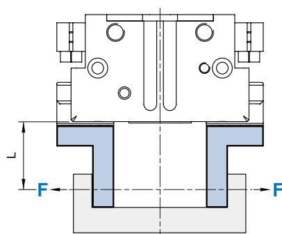
Internal grip
